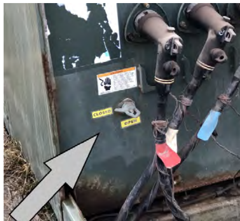
PIC 1. R7 Switchgear- Showing the switch in the closed (energized) state.
